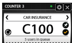
Virtual console
